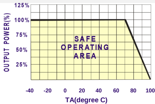
DERATING CURVE
