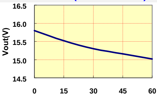
VOUT VS LOAD(15Vout Models)
